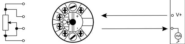
Resistance to 4-20 mA
