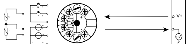
Resistance to 4-20 mA
