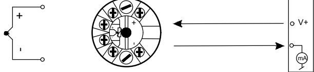
Thermocouple to 4-20 mA
