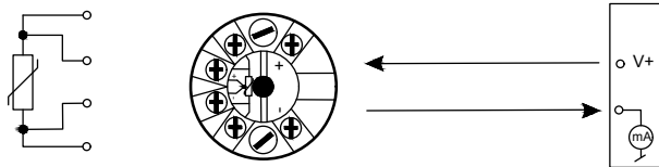
RTD to 4-20 mA
