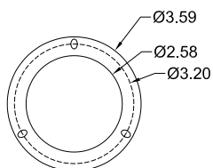
2.5" MOUNTING FLANGE
