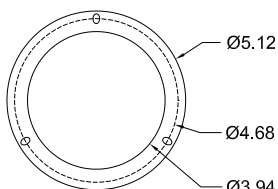
4" MOUNTING FLANGE
