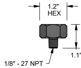
1/8" NPT
