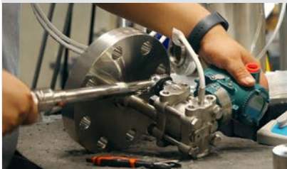
Diaphragm Seals
