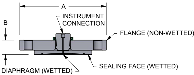
W9FR Rotating Flange
