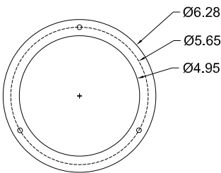
PT45T Mounting Flange
